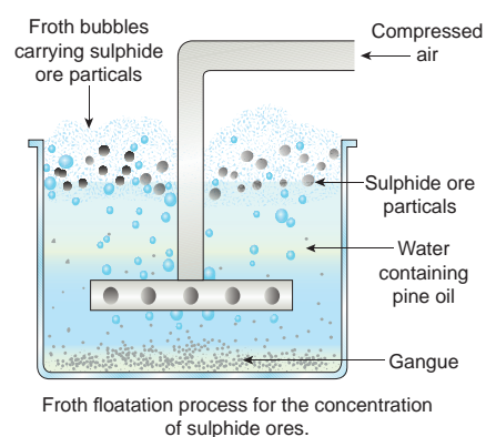
Figure 8.9 Froth floatation
